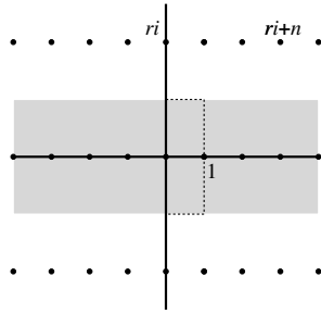
FIGURE 1.6. Degeneration of a lattice to the integral points on the real axis.
