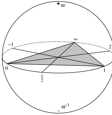
FIGURE 1.12. The \mathfrak{S}_3 -action on \mathbb{P}^1 through the dihedral group action.
